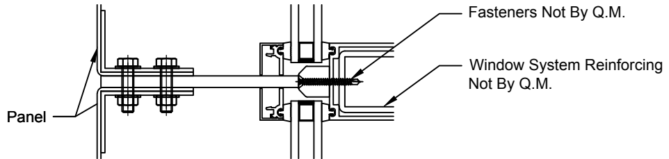
DETAIL AT MID-SCREEN ANCHOR
